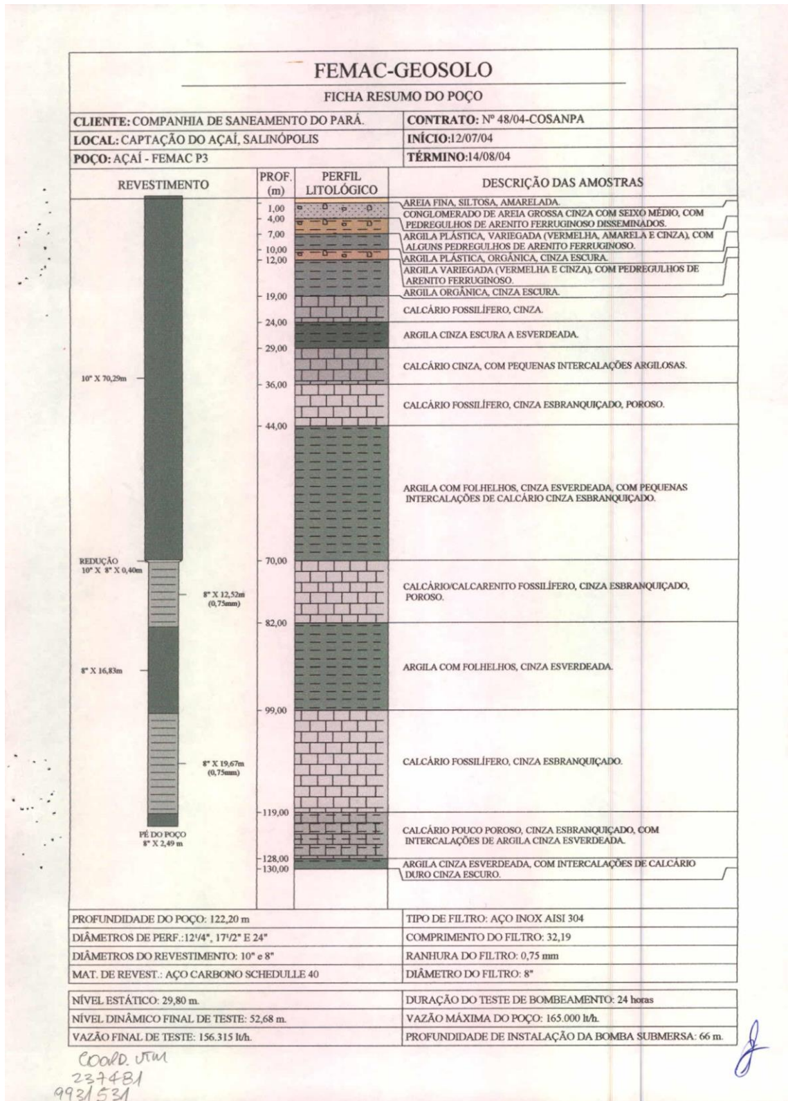
Figura 12 - Perfil construtivo do poço Açai Femac-P3 Figure 12 – Constructive profile of the well Açai Femac-P3
